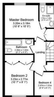
Second Floor
